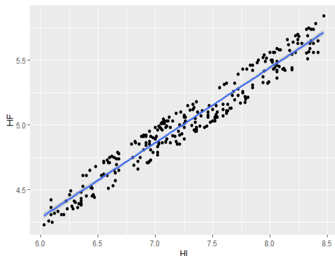
Figure 2: Regression Line
