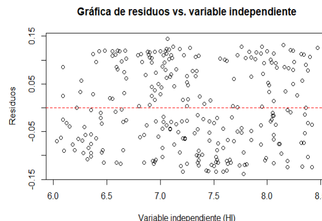
Figure 4: Residuals vs. Independent Variable Plot
